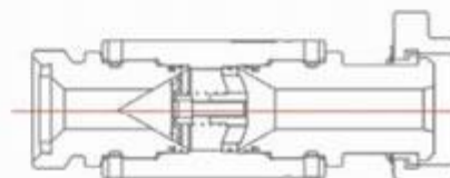
Dart style check valve
