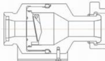
Flap check valve
